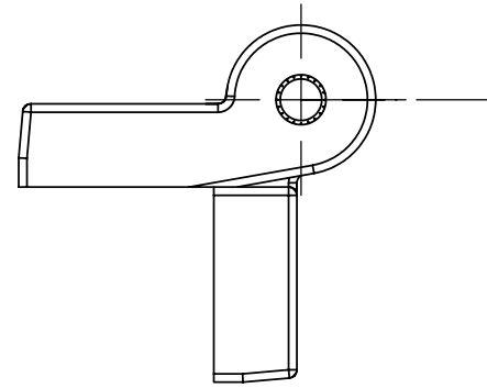
90° Fold
